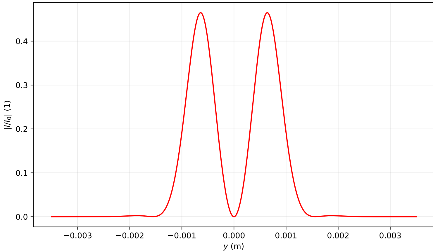
Intensity profile I(x=0, y, z=1.672)/I_0 , P_{in}=3.0P_{cr} , artificial time
